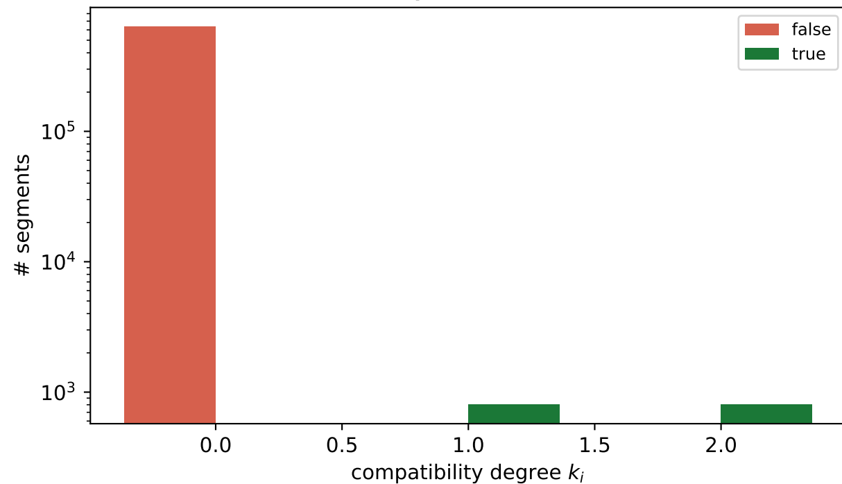
Event A (clean, \varepsilon=1\text{e-}6 ) coupled-false = 0
