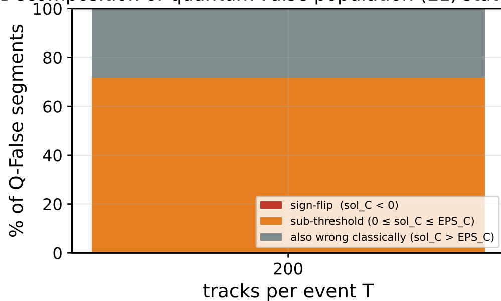
Decomposition of quantum-False population (E1, statevector)
