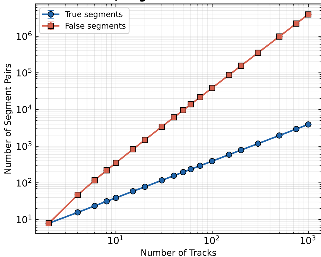
iii) Segment Pair Counts
