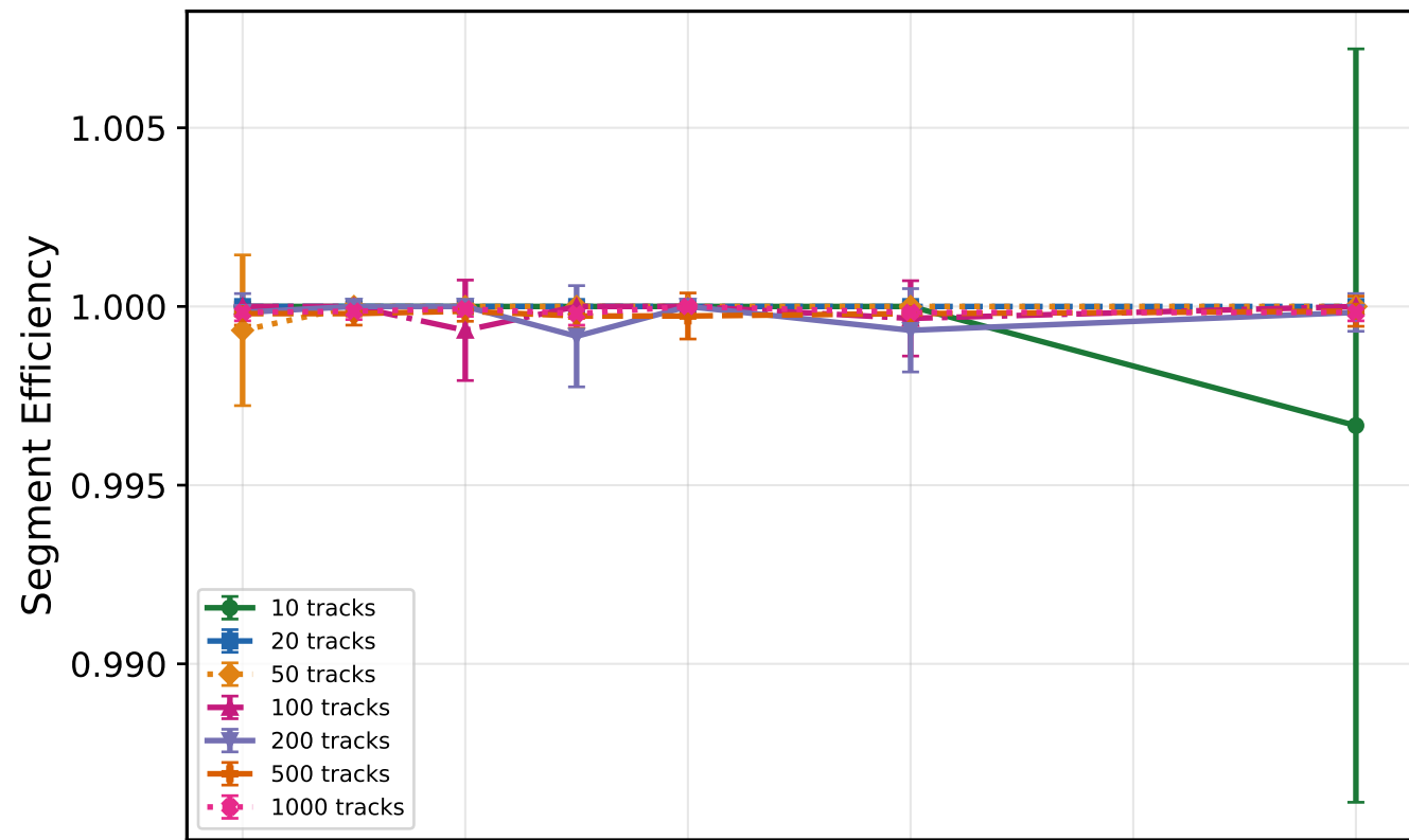
Segment metrics vs hit resolution ( \phi_{\text{max}} = \theta_{\text{max}} = 0.02 rad, \sigma_{\text{scatt}} = 0.10 mrad) Extended to 1000 tracks
