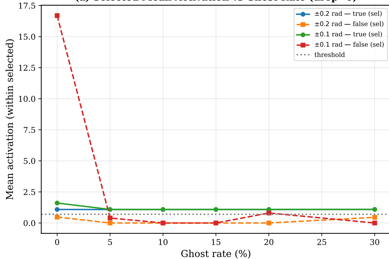
(a) Selected Mean Activation vs Ghost Rate (drop=0)
