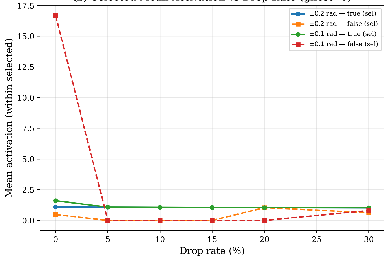
(b) Selected Mean Activation vs Drop Rate (ghost=0)
