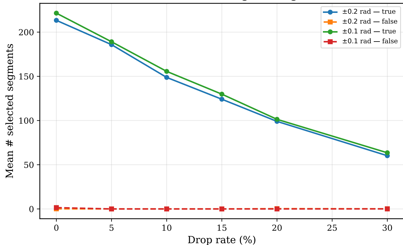
True vs False Selected Segments (ghost=0)
