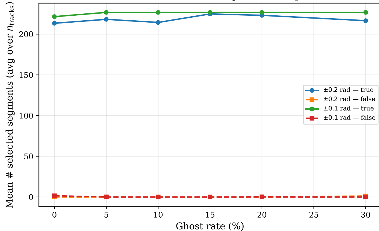
True vs False Selected Segments (drop=0)
