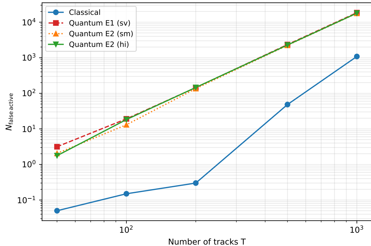
(b) False-active segment count (quantum activates many more)
