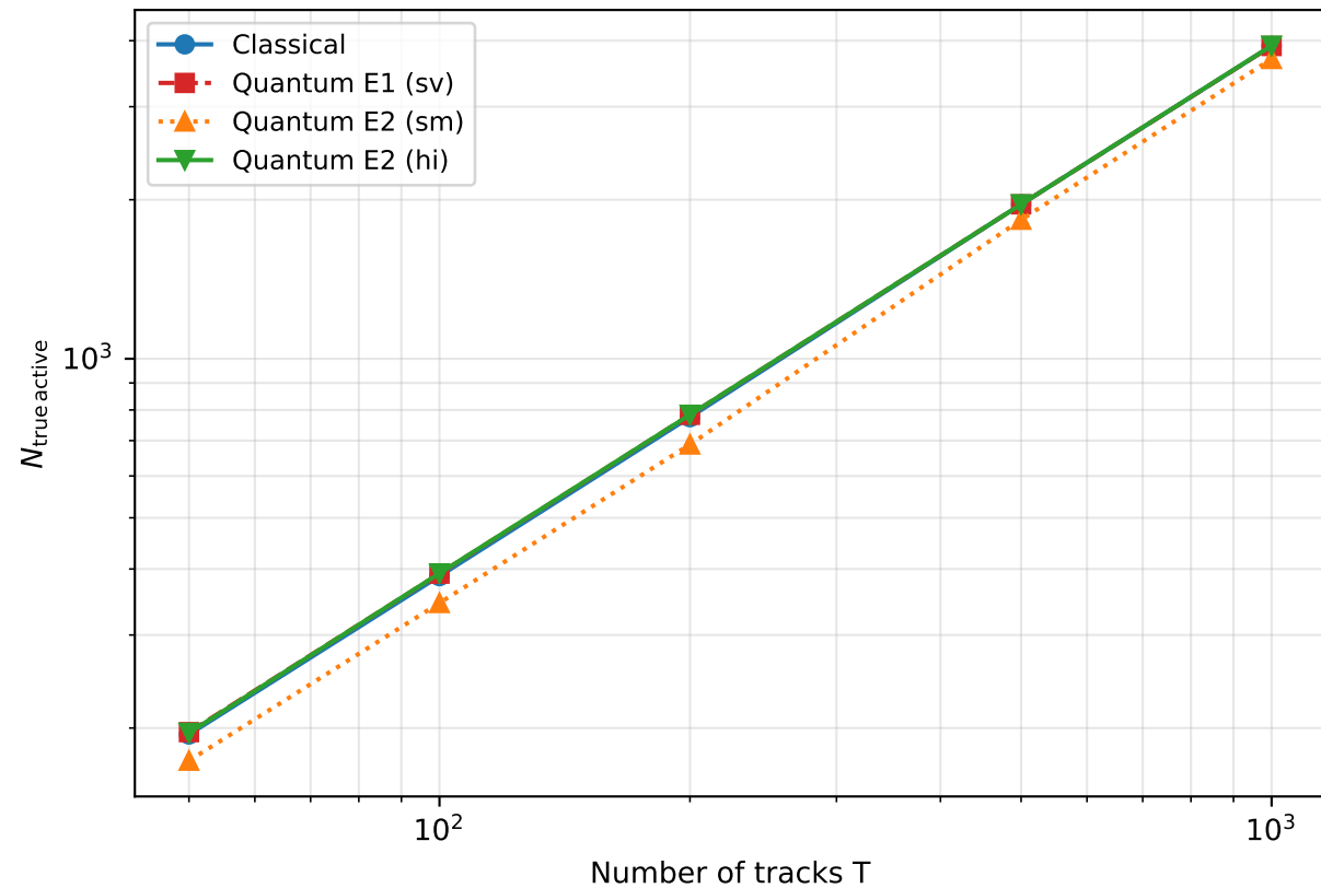
(a) True-active segment count (classical and quantum coincide)
