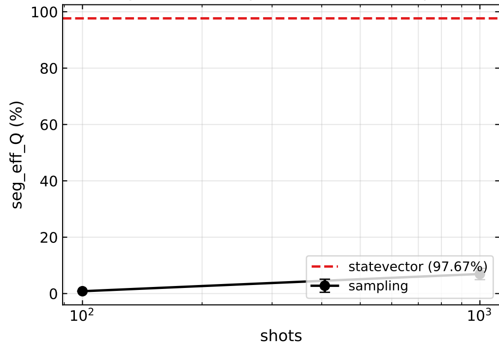
a) Segment efficiency vs shots ( T=30 , drop=1%)
