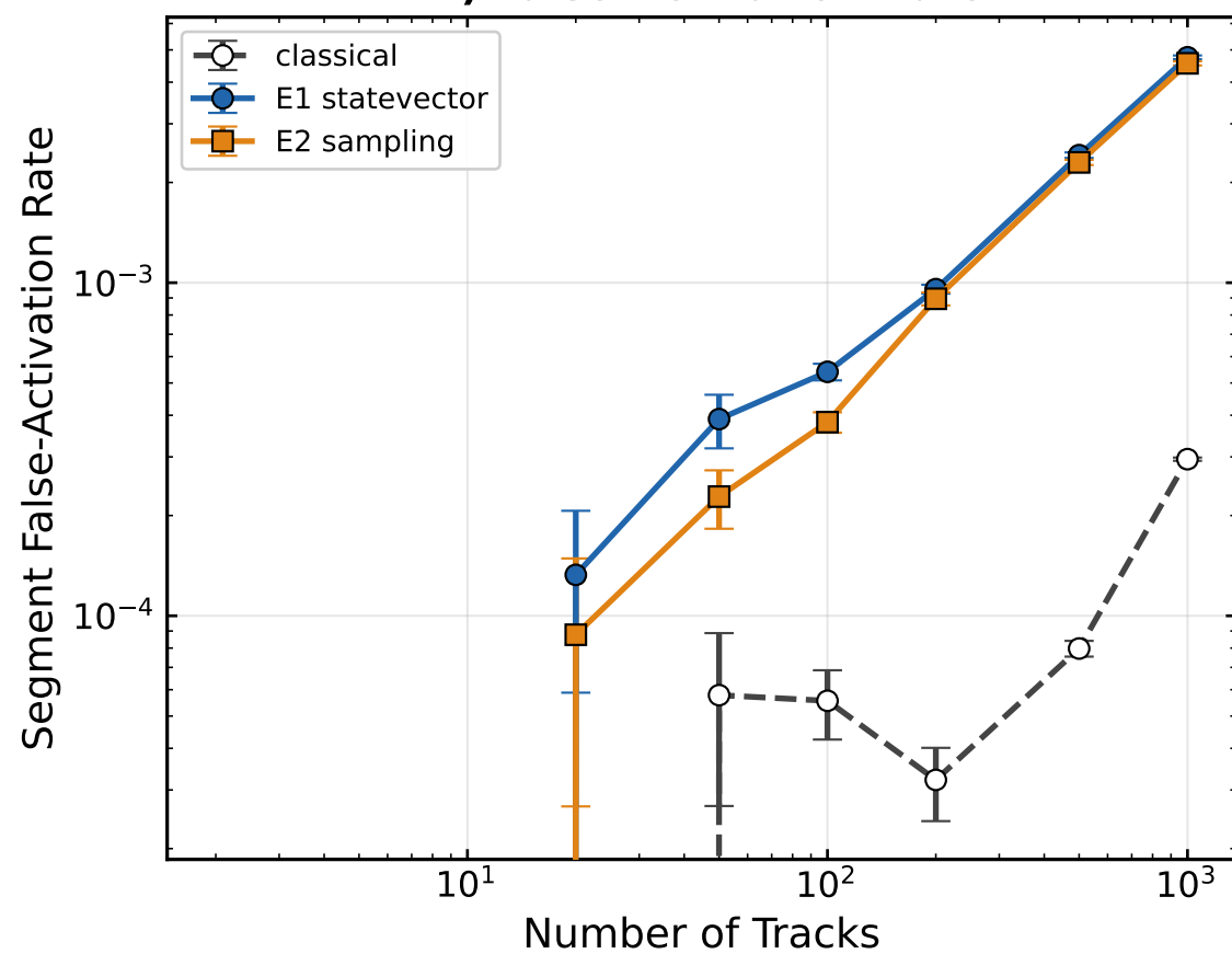
iii) False-Activation Rate
