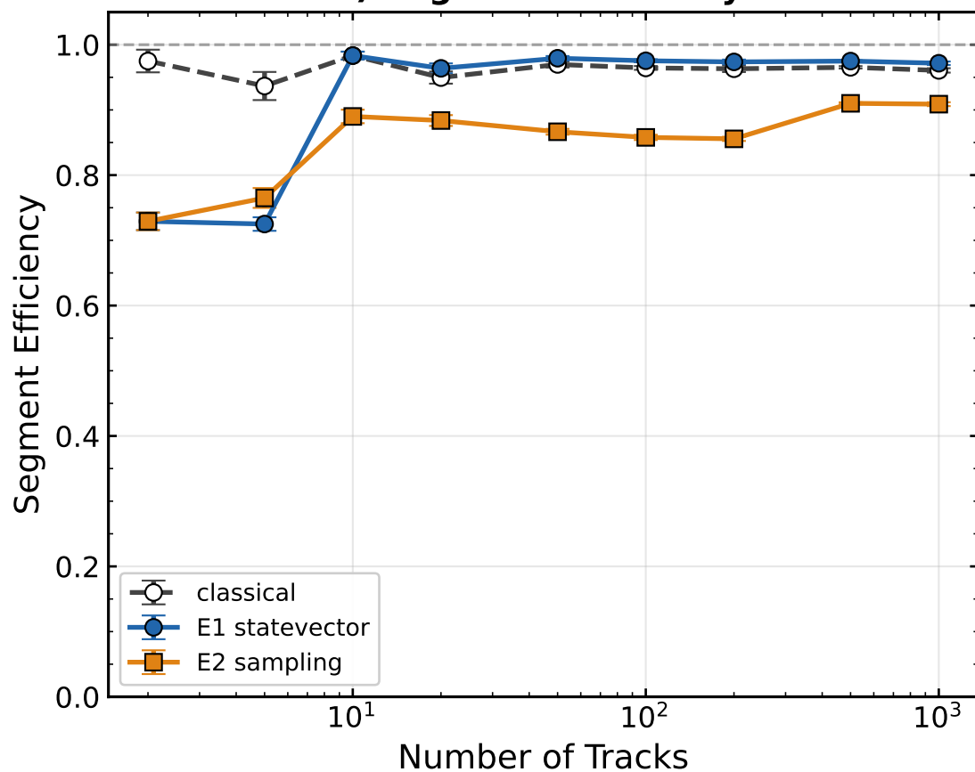
i) Segment Efficiency
