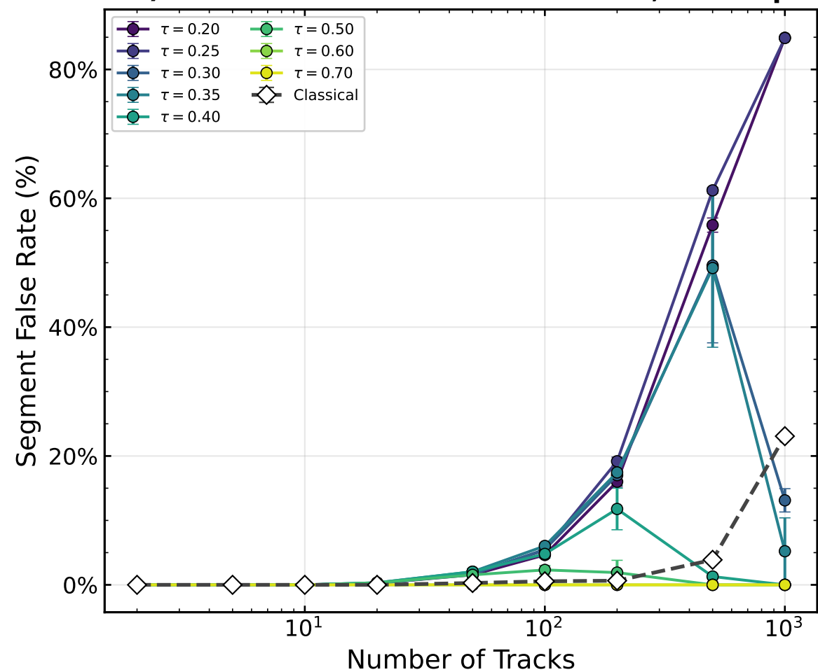
ii) False Rate vs T — E1 statevector, \tau -sweep
