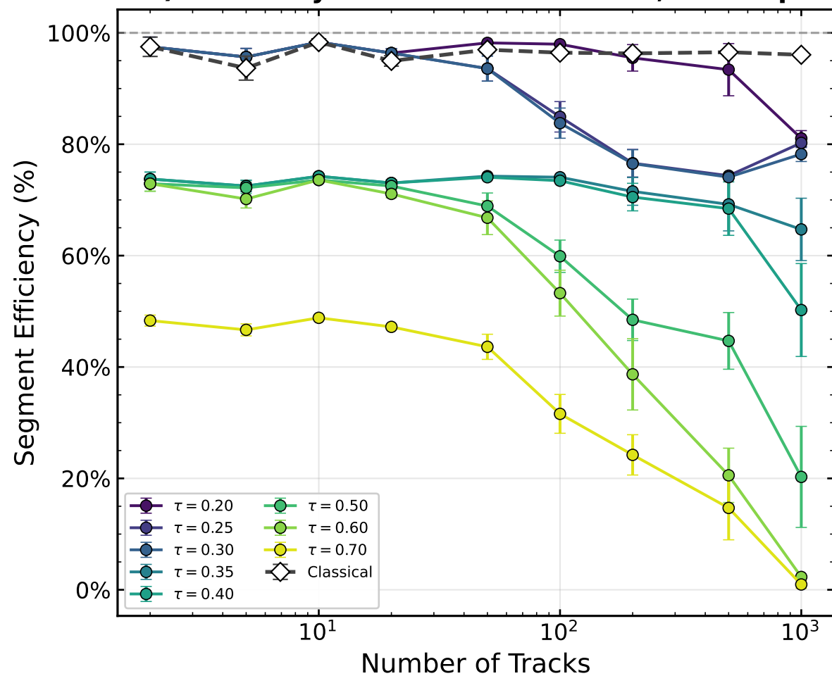
i) Efficiency vs T — E1 statevector, \tau -sweep
