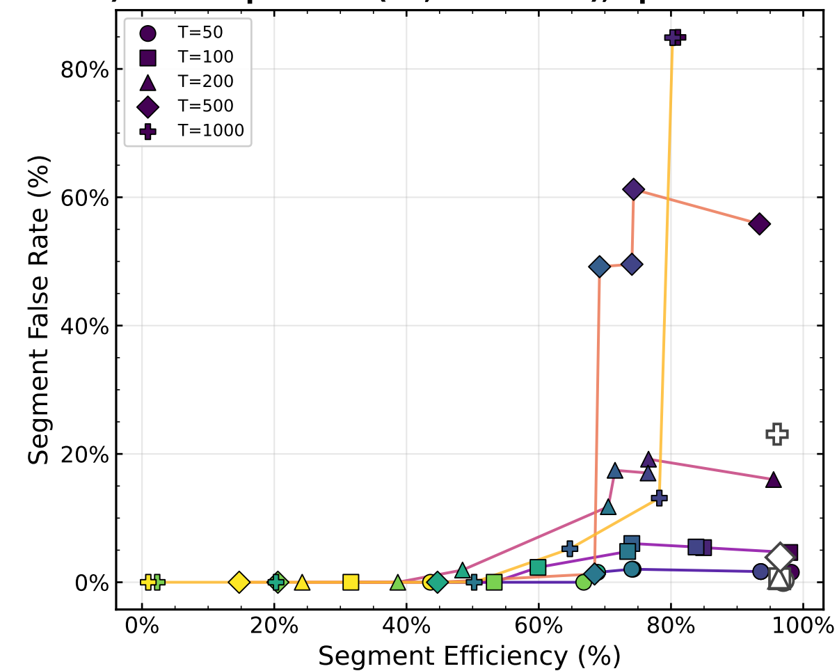
iii) ROC — quantum (E1, colour = \tau ), open = classical
