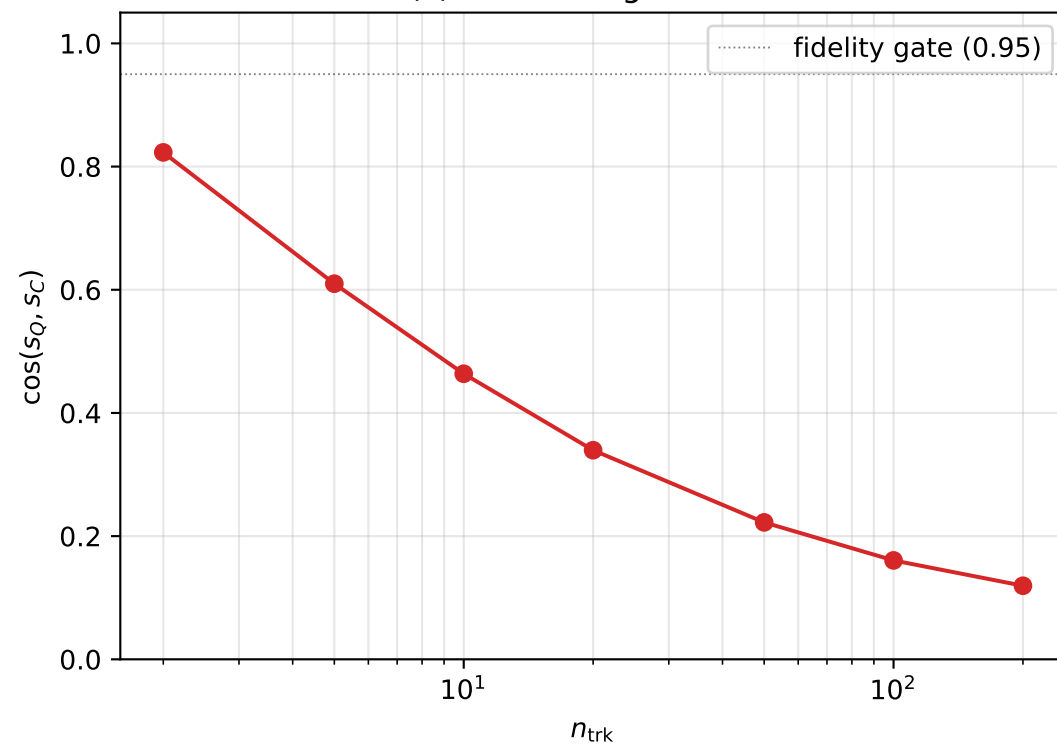
(c) Solution agreement
