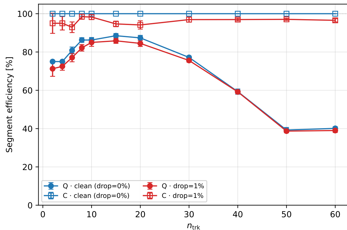
Quantum (1BQF) vs classical segment-level active metrics — threshold \tau=0.35 , condor pickles
