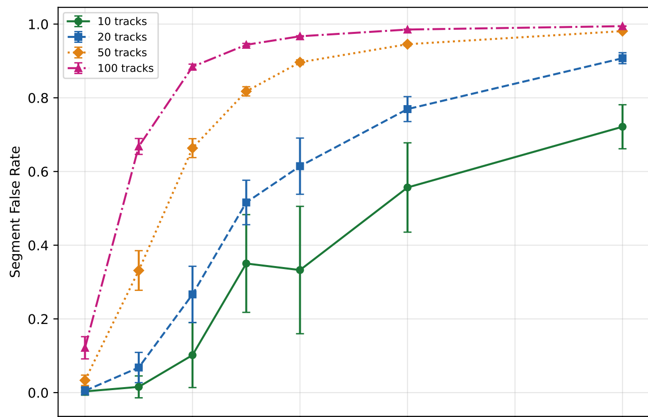
Segment metrics vs hit resolution ( \phi_{\text{max}} = \theta_{\text{max}} = 0.02 \text{ rad} , \sigma_{\text{scatt}} = 0.10 \text{ mrad} )
