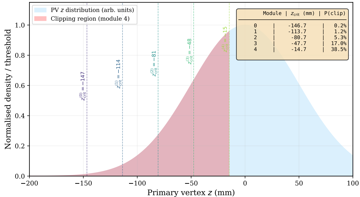
Figure 2: PV z Distribution vs Module Clipping Thresholds ( \phi_{\text{max}} = 0.2 rad, detector half-width = 50.0 mm)
