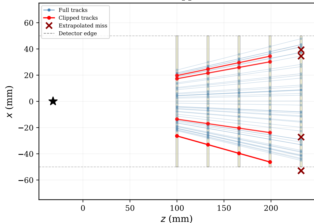
(a) Event display — PV z = -31.8 mm 45 full + 5 clipped tracks
