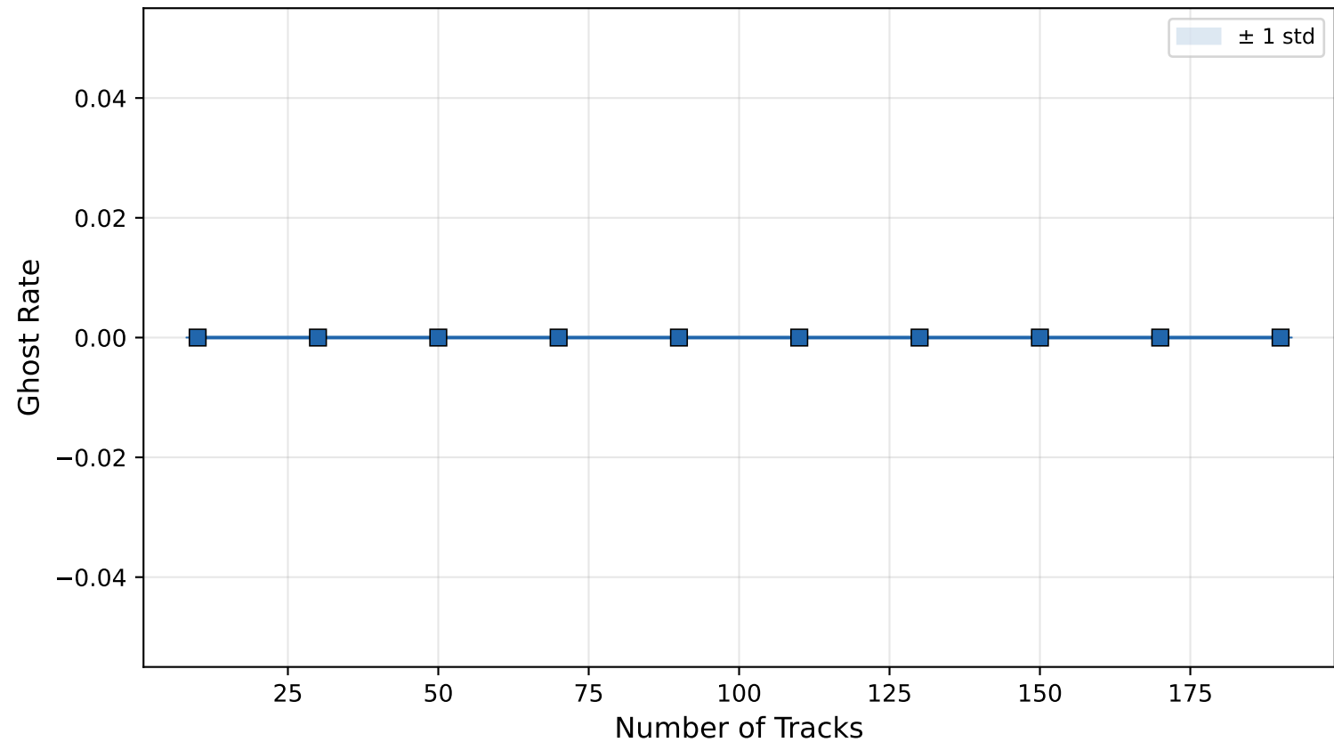
Ghost Rate vs Event Size ( \sigma_{\text{scatt}} = 0.1 \text{ mrad} , \sigma_{\text{res}} = 5 \mu\text{m} , \gamma = 3.0 )
