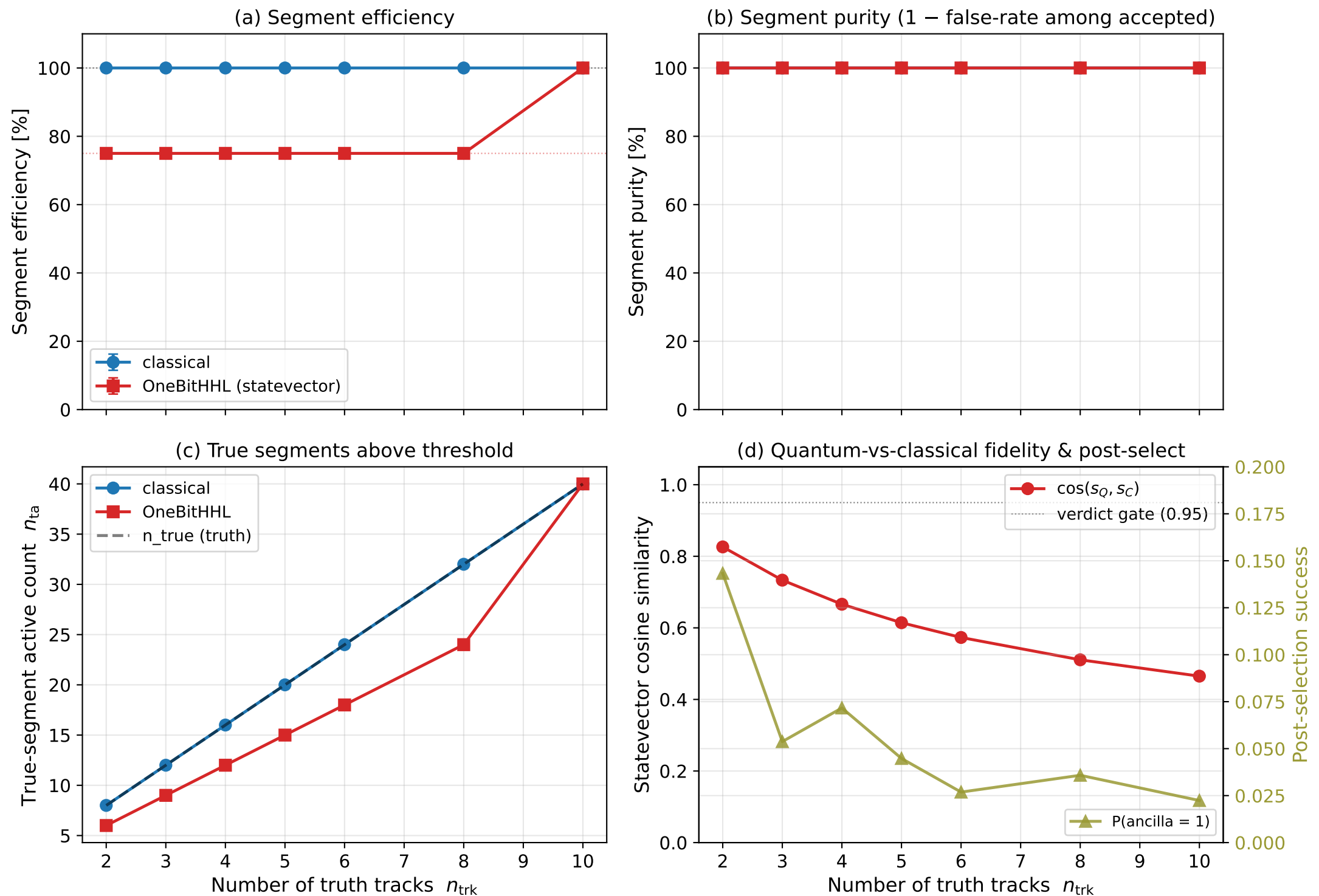
OneBitHHL segment-level fidelity vs n_{\text{trk}} ( \tau=0.35 , statevector — no shot noise, 5 reps/n)
