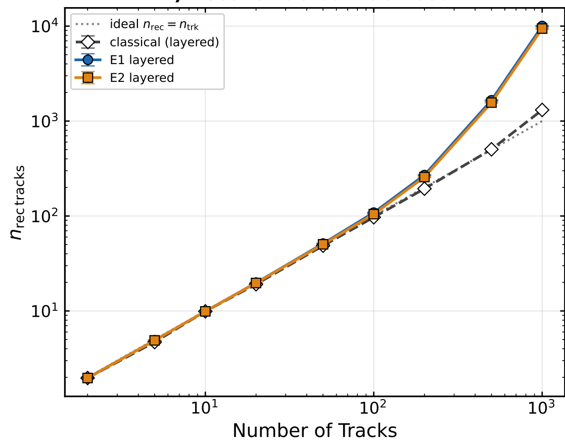
iv) Reconstructed-Track Count
