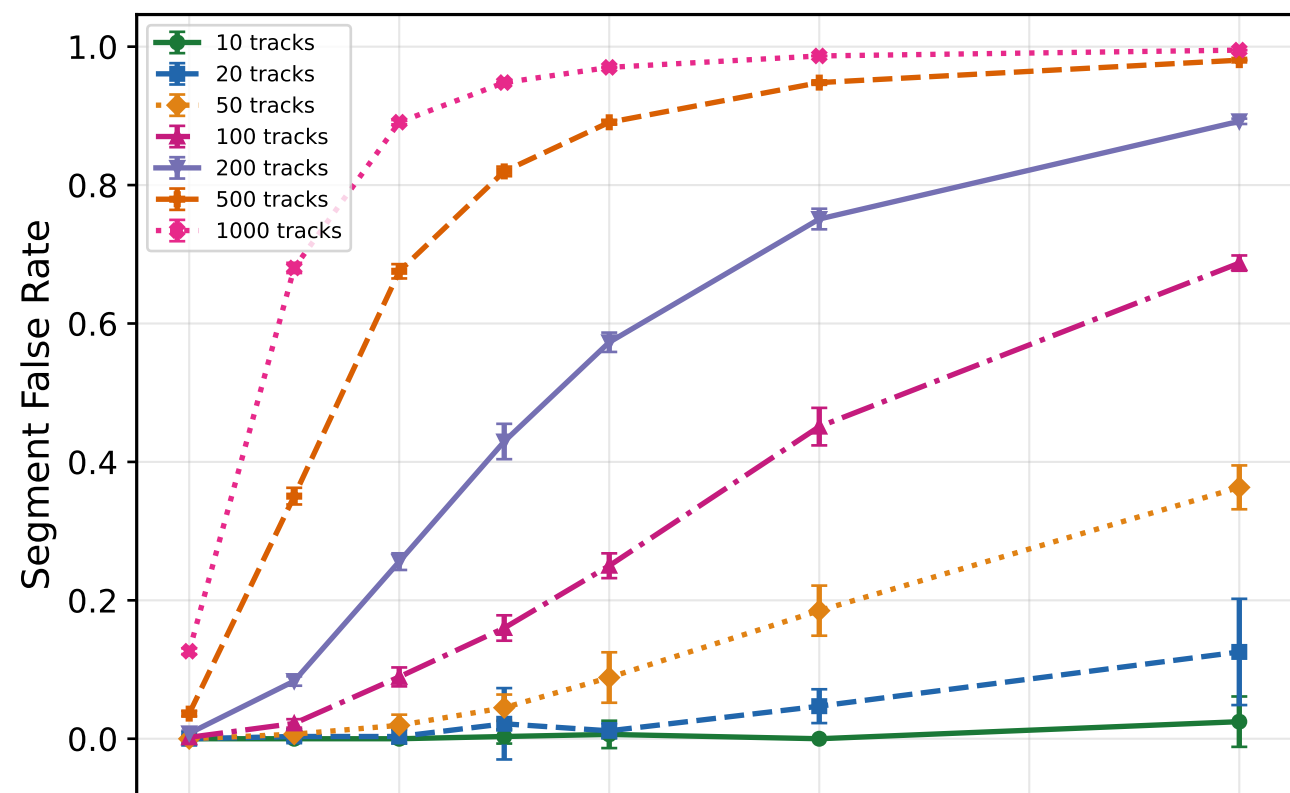
Segment metrics vs hit resolution ( \phi_{\text{max}} = \theta_{\text{max}} = 0.2 \text{ rad} , \sigma_{\text{scatt}} = 0.10 \text{ mrad} ) Extended to 1000 tracks
