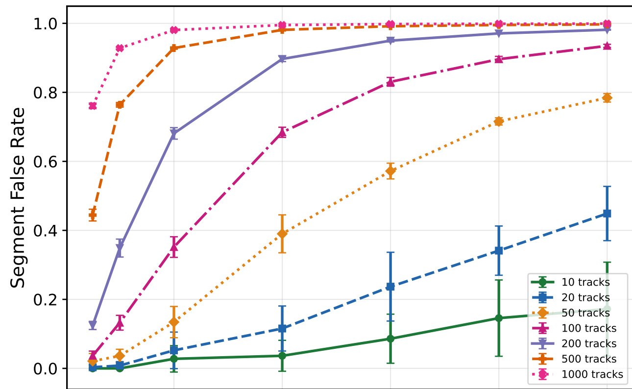
Segment metrics vs scattering ( \phi_{\max} = \theta_{\max} = 0.02 rad) Extended to 1000 tracks
