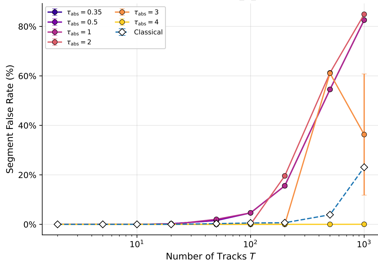
(a) Absolute \tau on sol_Q_scaled
