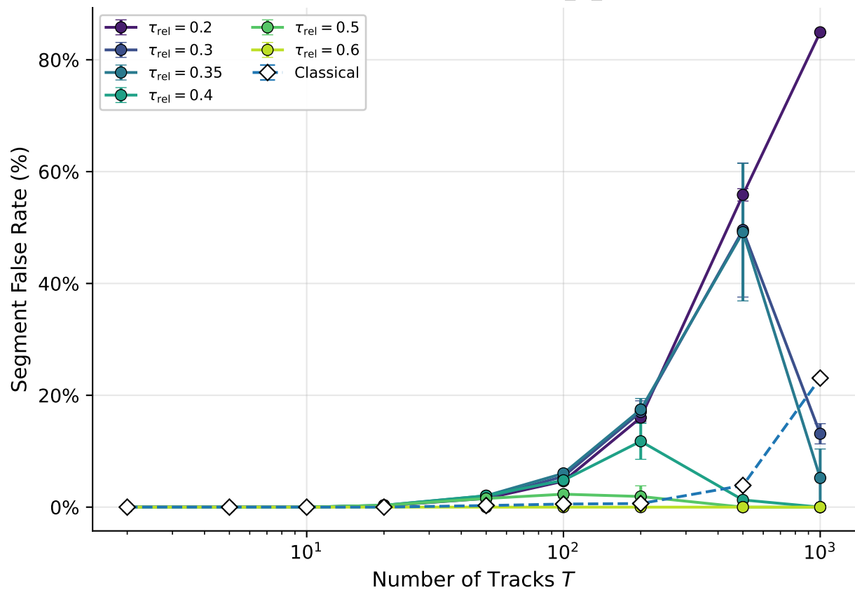
(b) Relative \tau \cdot q_{\text{max}} on sol_Q_scaled
