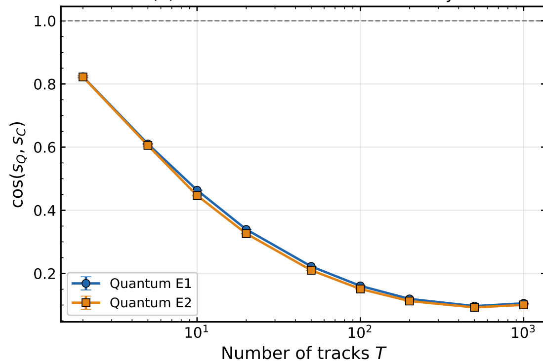
(a) Solution-vector cosine similarity
