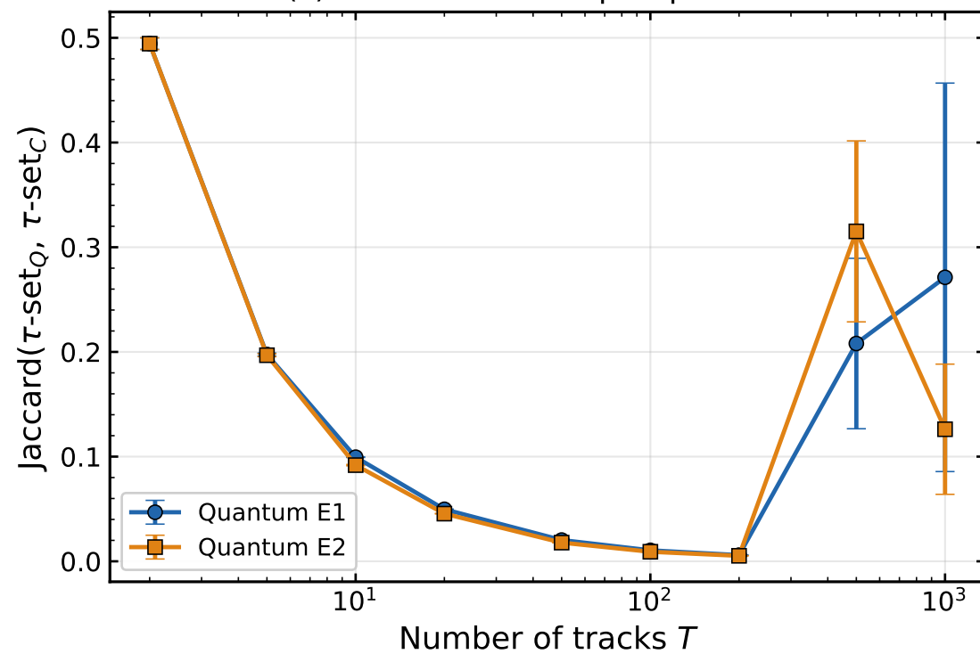
(c) Activation overlap at perfect \tau
