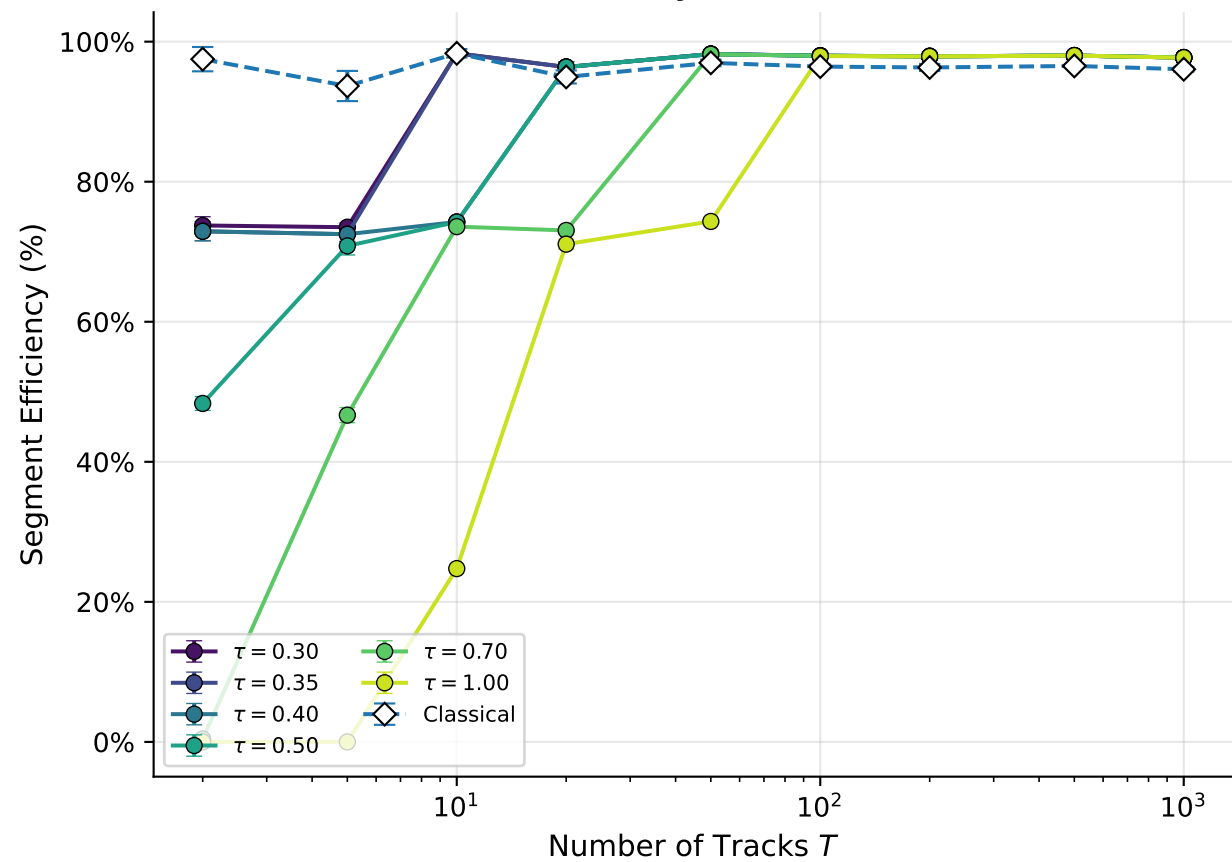
(b) Quantum efficiency vs T at absolute \tau (E1)
