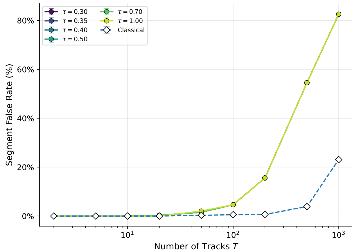
(a) Quantum FR vs T at absolute \tau (E1)
