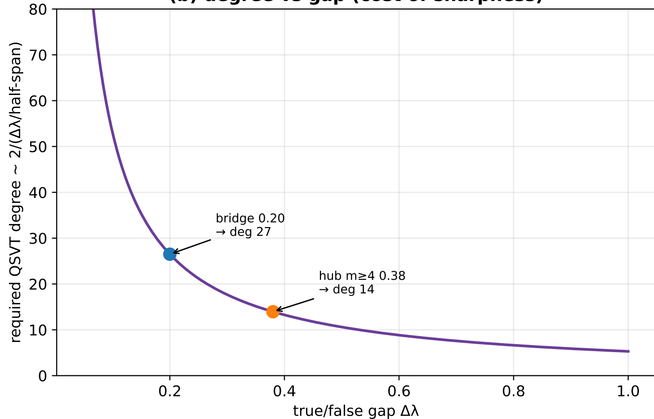
(b) degree vs gap (cost of sharpness)
