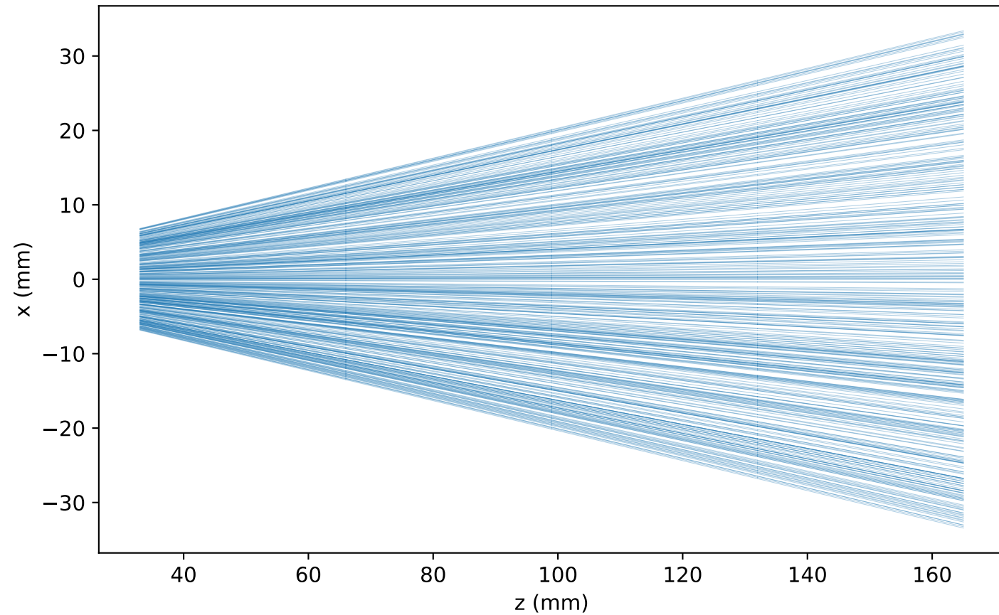
(a) The 400-track event (each faint line = one true segment)
