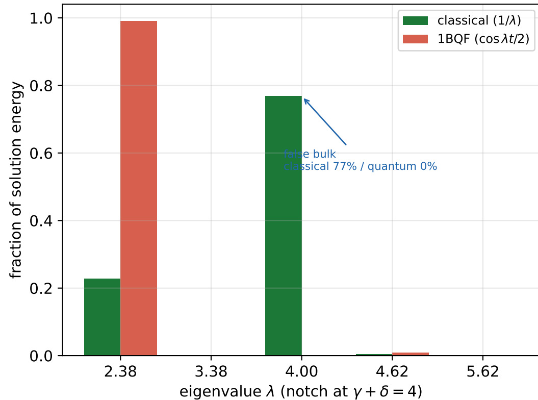
(b) Where each solver's solution lives in the spectrum
