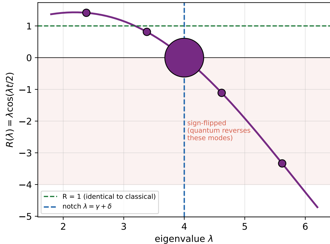
(a) Quantum-vs-classical re-weighting per mode
