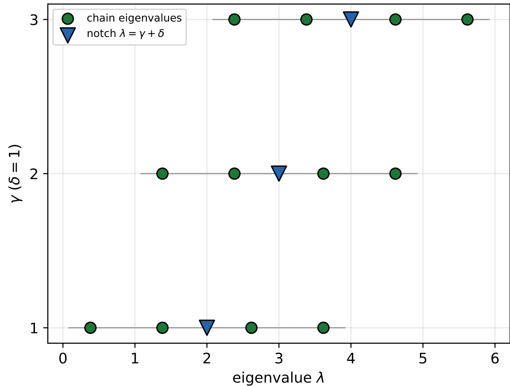
(c) The notch bisects the chain spectrum for every \gamma
