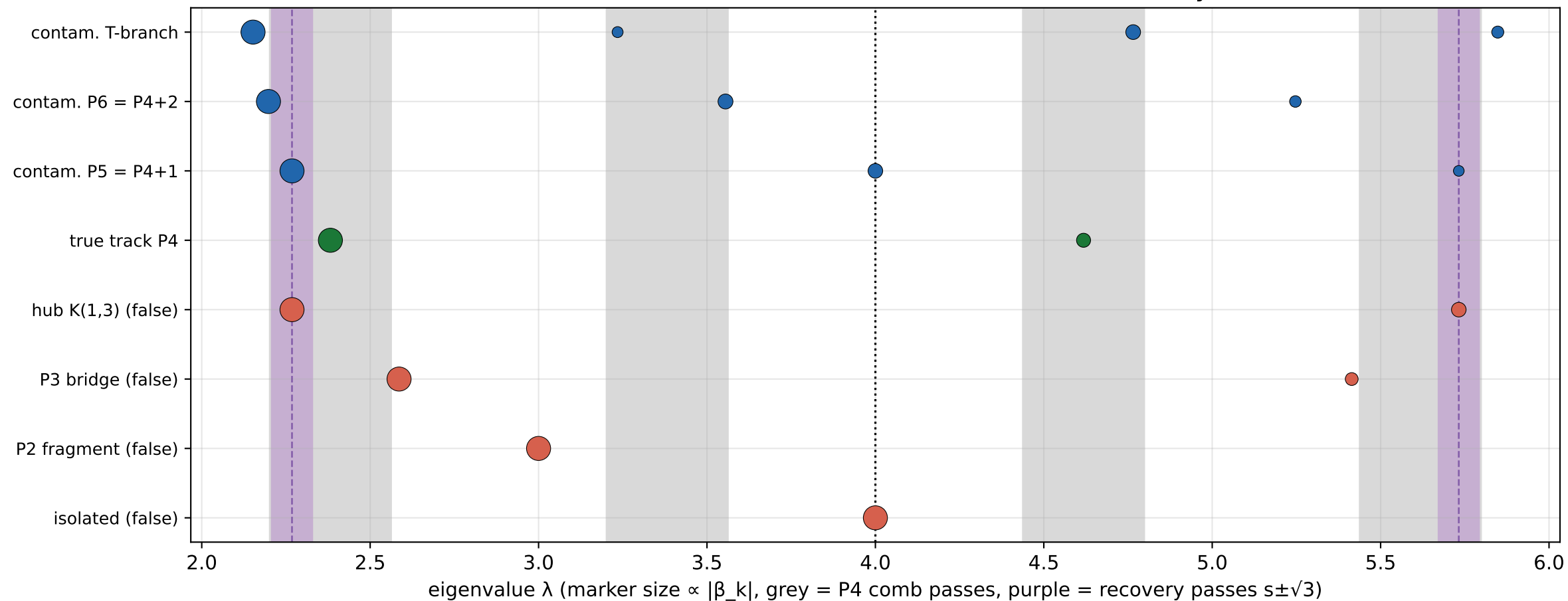
The line atlas: contaminated-P5 odd lines \equiv hub K(1,3) lines, exactly at s \pm \sqrt{3}
