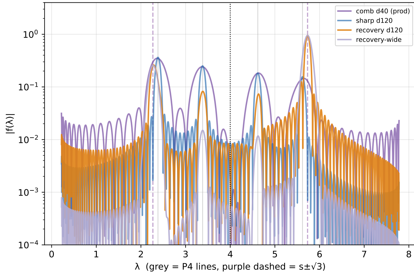
(a) the filter responses
