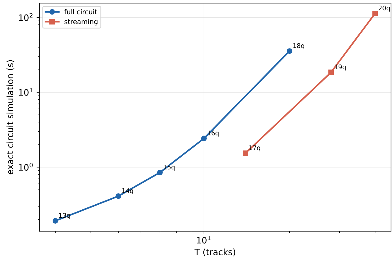
(b) local explicit-circuit cost (dense walk operator)
