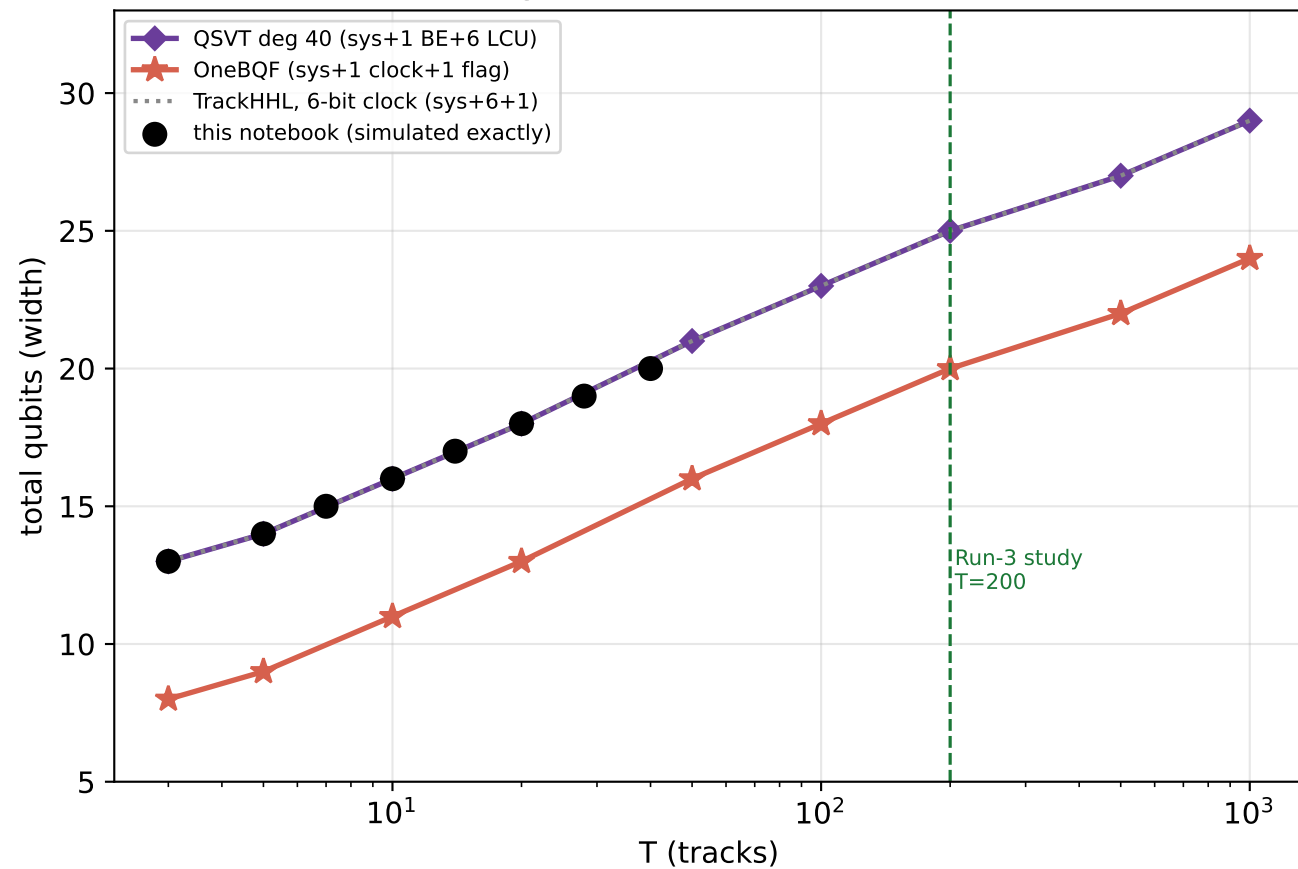
(a) qubit scaling: width is cheap — 29 qubits at T=1000
