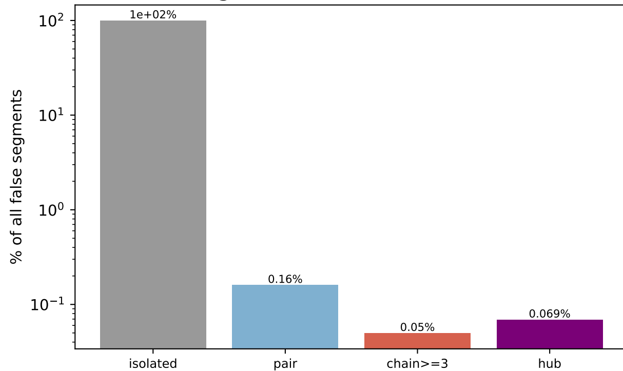
(a) False-segment census (all 99.7% are isolated)
