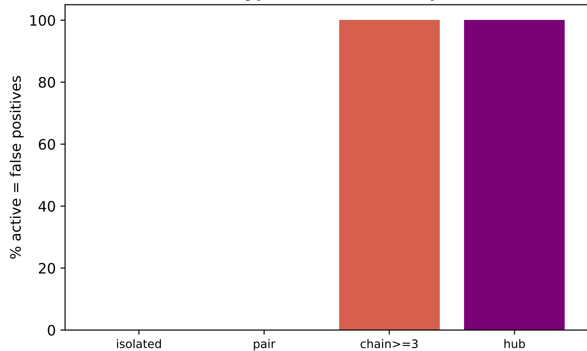
(b) Which types become false positives
