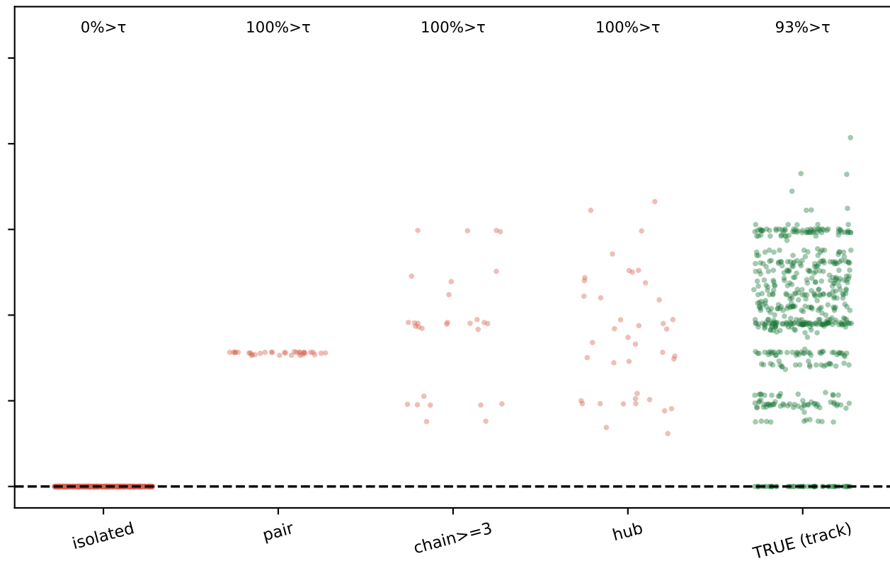
QUANTUM ( \cos \lambda t/2 , wp99 \tau=0.00 )
