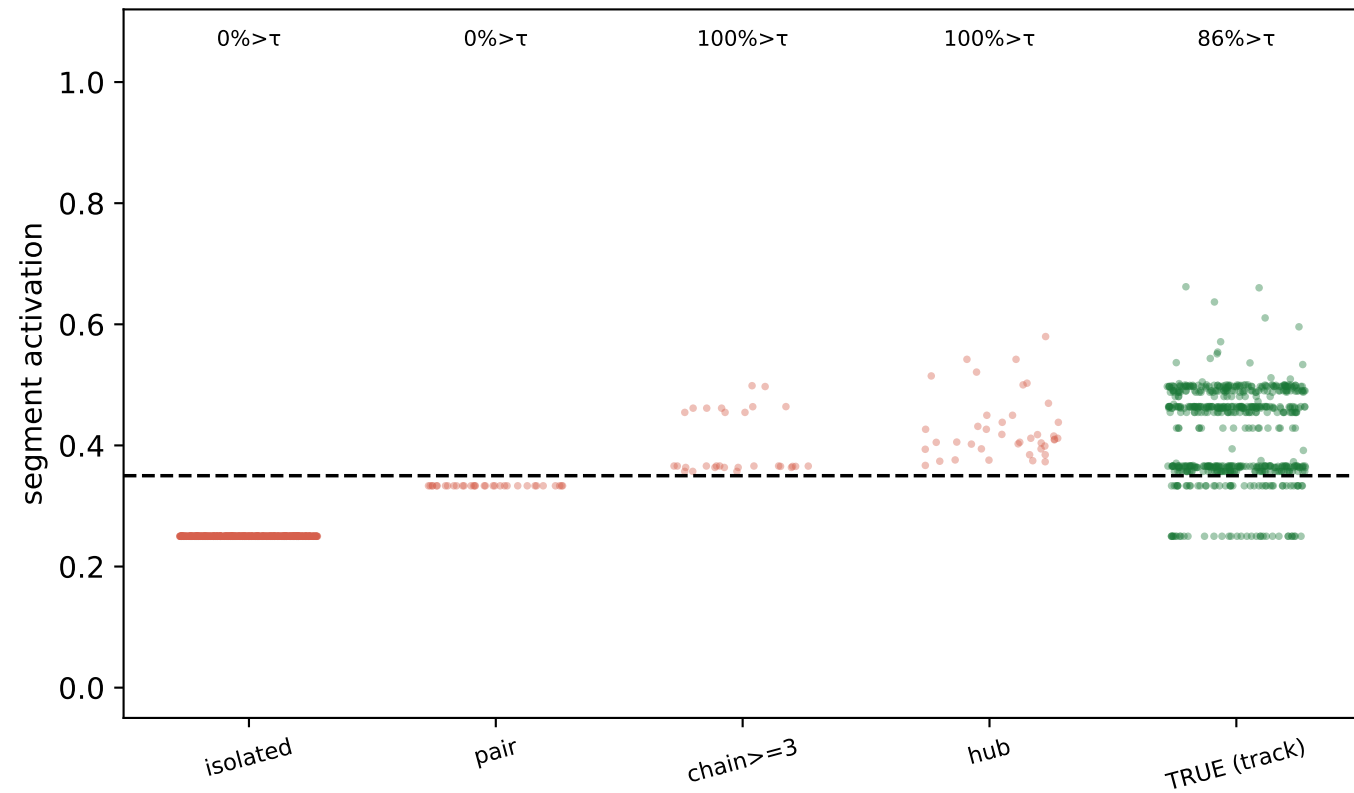
CLASSICAL ( 1/\lambda , \tau=0.35 )
