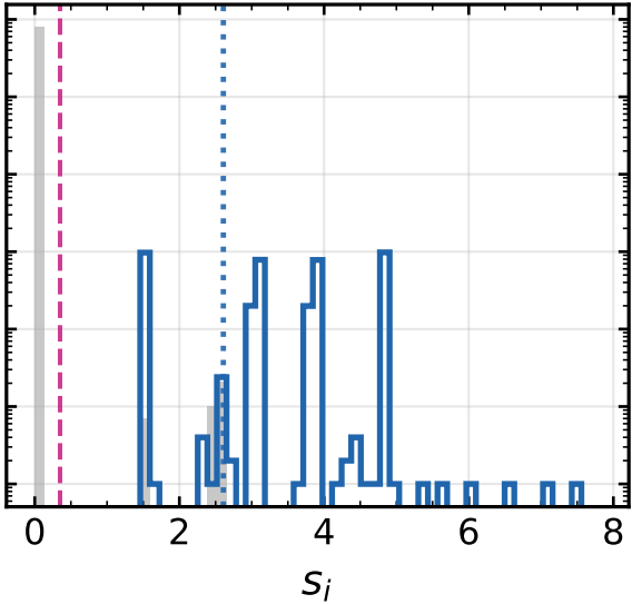
ii) Quantum (scaled), T=200
