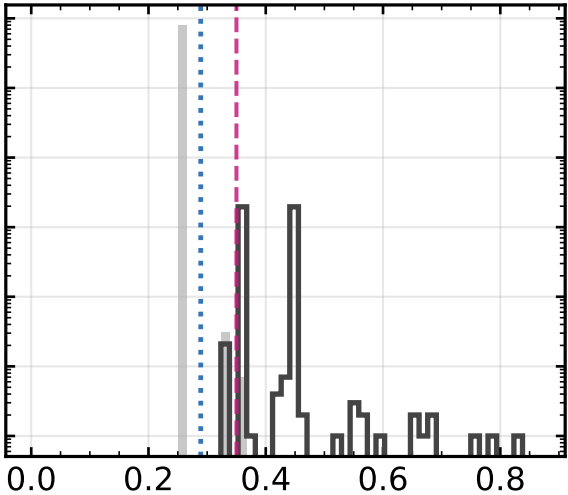
ii) Quantum (scaled), T=200
