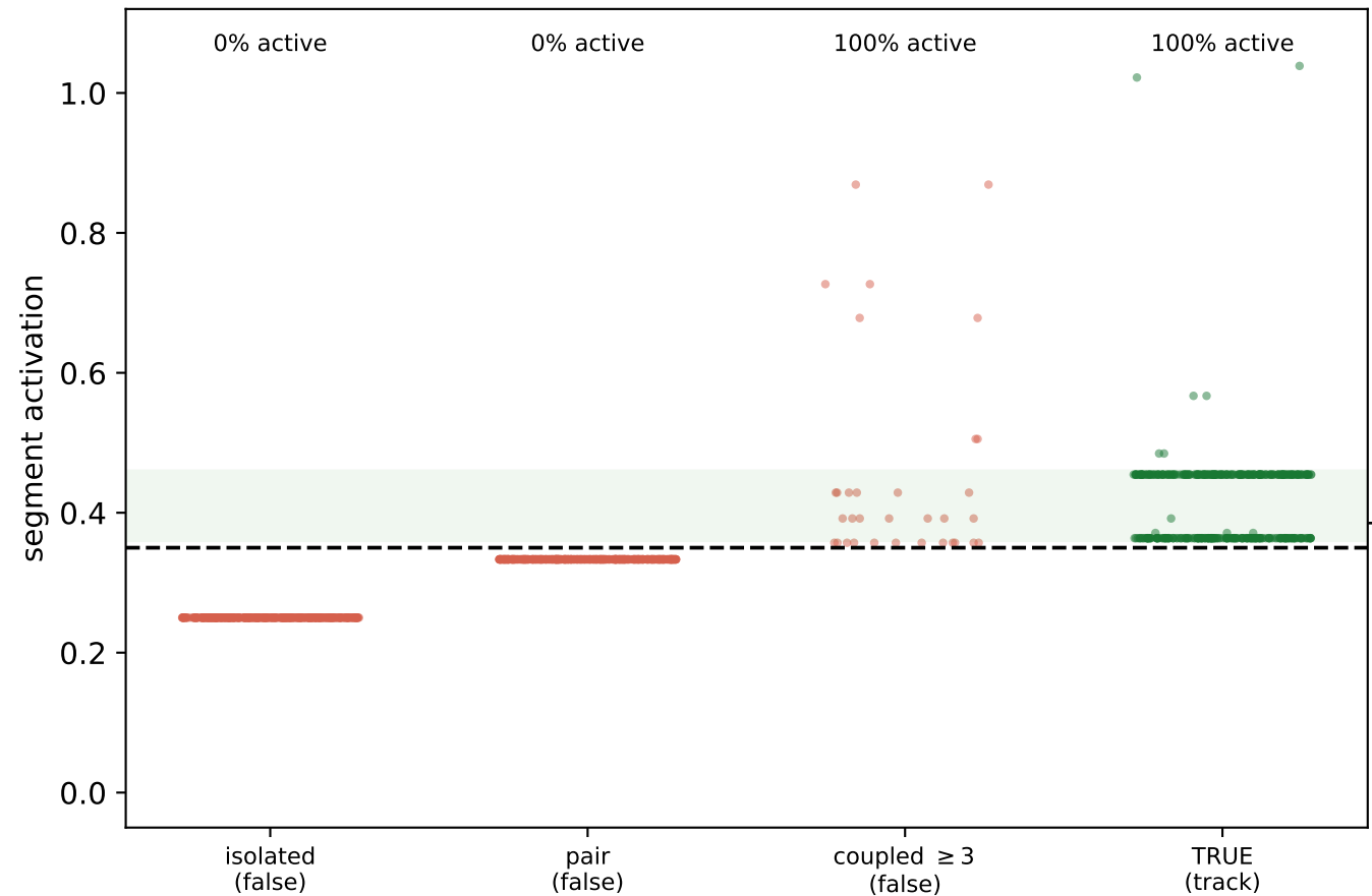
CLASSICAL ( 1/\lambda )
