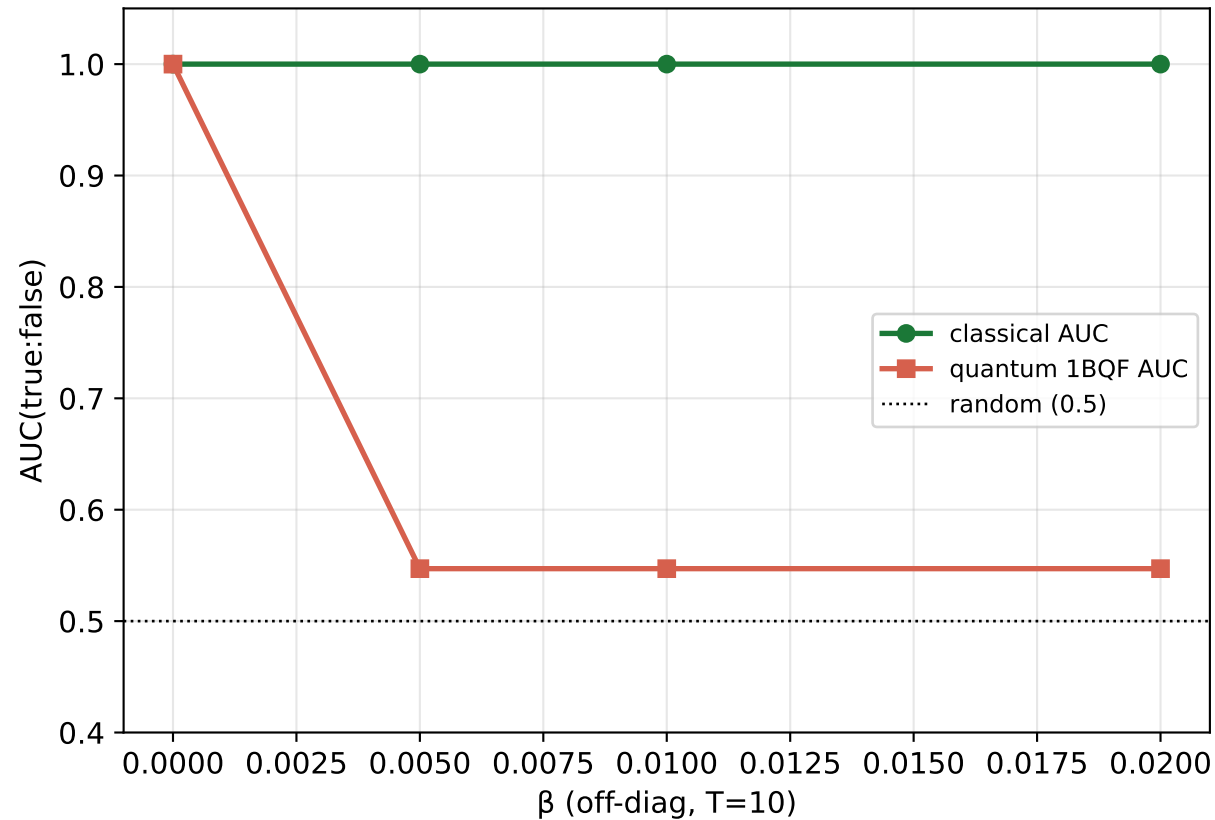
(a) Quantum discrimination collapses; classical intact
