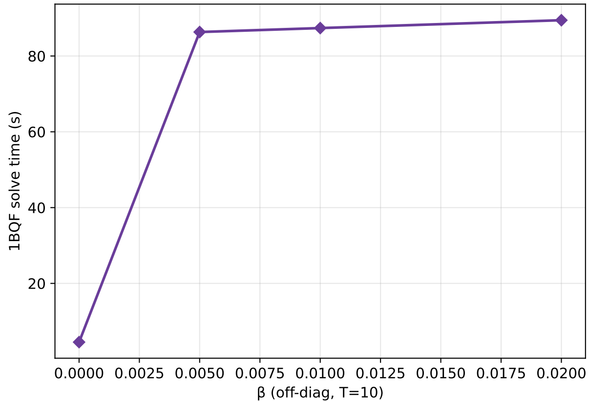
(b) Dense fork circuit: \sim 20\times slower at \beta > 0
