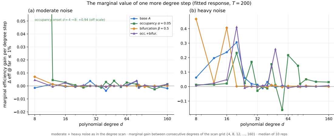
Figure 17: The marginal value of one more degree step (the derivative of the sigmoids of figures 15–16). (a) Moderate: after occupancy’s onset step (+0.94 from d=4 to 8, off scale) every operator’s marginal gain is consistent with zero at every degree. (b) Heavy: the marginal gain peaks at the operator’s onset and decays to zero past it, with the non-monotone ripple of the fitted family visible as negative excursions.
