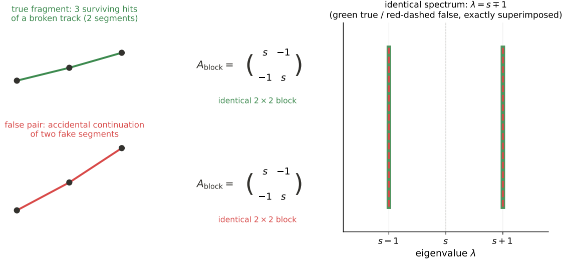
Figure 8: Spectral twins. A true fragment of a broken track (top) and an accidental false pair (bottom) have isomorphic compatibility graphs, hence identical 2 \times 2 sub-blocks of A , hence exactly the same eigenvalues and amplitudes. Every function of A treats them identically; this is the floor theorem, and under noise it becomes the fragment floor of section 9.
