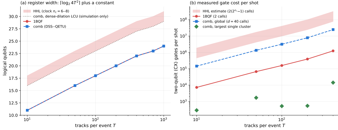
Figure 22: The rows of table 3 against track count. (a) Logical register width: all constructions follow \lceil \log_2 4T^2 \rceil plus a constant: the 1BQF and DSS-QETU comb lines coincide exactly (the comb pays no width for its degree on this primitive), while the dense-dilation LCU pays +5 and the HHL clock band +7 to +9. (b) Measured two-qubit gate cost per shot: the shared evolution call grows as \approx T^{1.4} (pair count \times ladder length), the three algorithms sitting at fixed multiples of it (2, 40, \approx 130 –510 calls). The green diamonds are the largest single per-cluster instance at each T : set by the local cluster size, not by T , the flat exception to every other curve’s growth.
