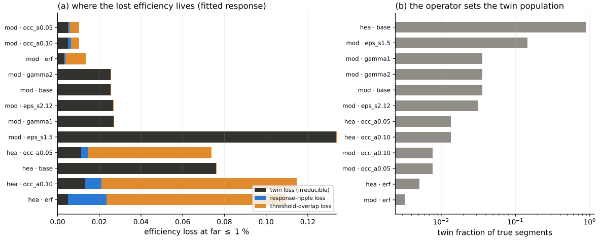
Figure 20: (a) The efficiency lost at the 1% false-rate budget, per operator (fitted response at its best degree), decomposed into its three named channels: twin loss, ripple loss, and threshold-overlap loss. On base A the entire deficit is twin loss — spectral twins, irreducible for any response. (b) The twin fraction of true segments per operator (log scale): the operator sets the twin population; the response cannot touch it.
