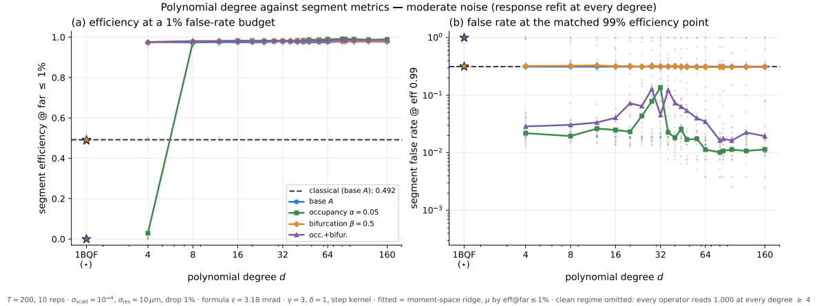
Figure 15: Polynomial degree against the two segment metrics on moderate noise ( T=200 , ten repetitions; per-repetition dots, median lines; response refitted at every degree). Stars at the left edge: the matched 1BQF, a degree-one filter, on each operator. (a) Efficiency at a 1% false-rate budget: every operator is flat from d \approx 8 — the response axis is exhausted almost immediately, at 0.975–0.978 on base A against the classical 0.492. (b) False rate at the matched 99%-efficiency point: base A and the fork sit pinned at the 0.31 twin flood at every degree, while the occupancy operators alone drop to the 10^{-2} scale — purity at high efficiency is bought by the operator, not the polynomial.
