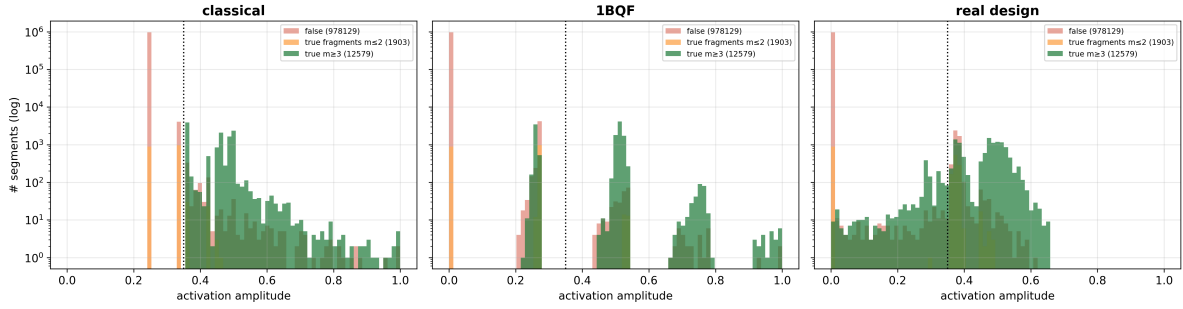
Figure 24: The real-geometry counterpart of the toy's amplitude pile-up: activation-amplitude spectra on real Run-3 VELO event geometry, for the classical solver, the 1BQF, and the redesigned band-plus-notch response. Pink: false segments; orange: true fragments ( m \leq 2 ); green: findable true segments ( m \geq 3 ); the dotted line is the fixed threshold. Variable track length smears the discrete toy levels into bands, and the fragment population sits inside the false bulk for every solver, the real-geometry form of the fragment floor.
