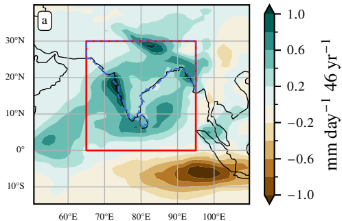
Summer precipitation trend
