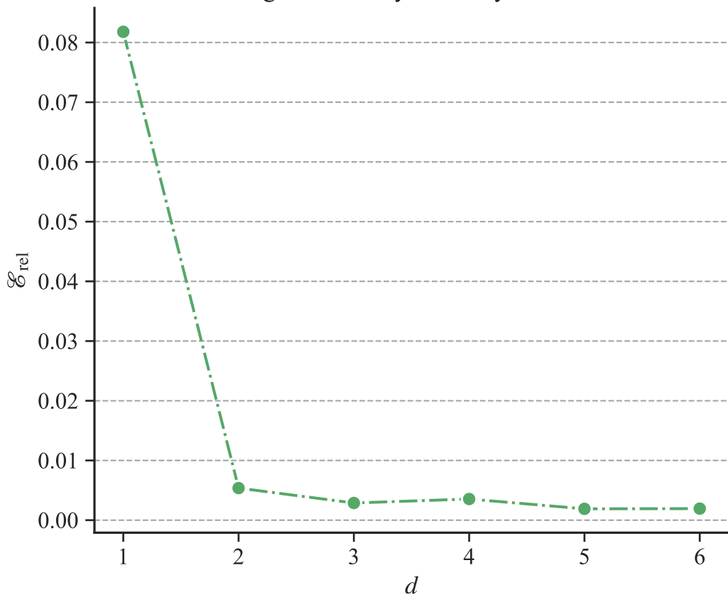
Degree of Chebyshev Polynomials
