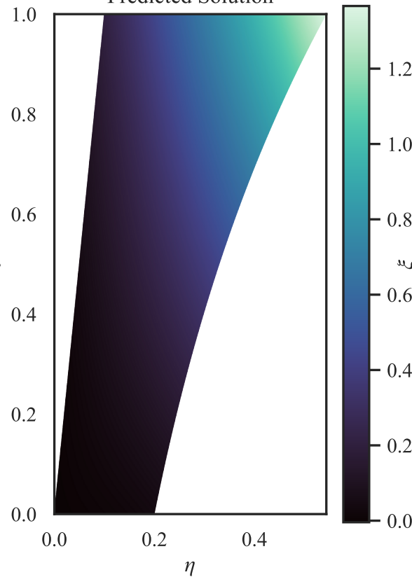
Predicted Solution
