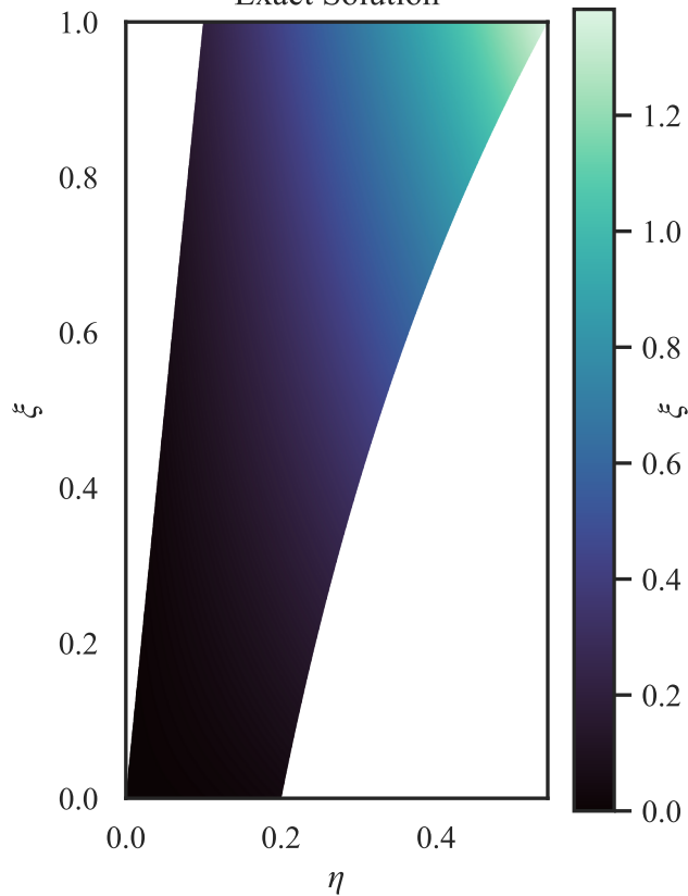
Exact Solution
