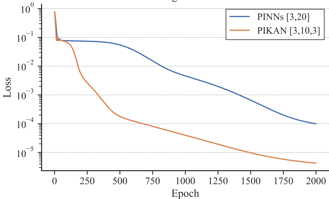
Training Loss Curve
