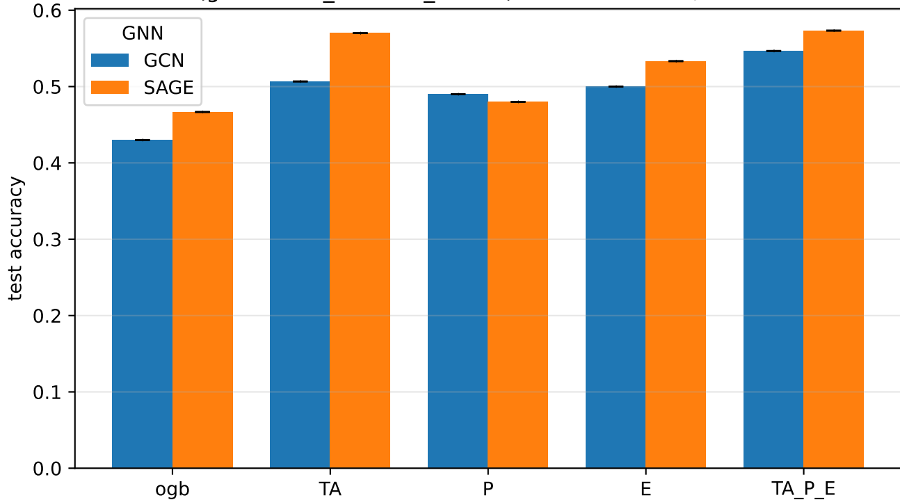
E2 (goodreads_children_n1500): feature \times GNN, n=1 seed
