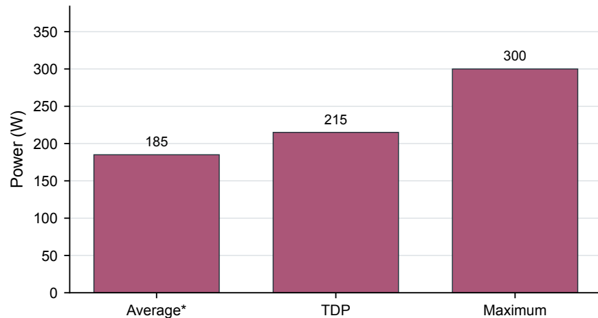
(d) GroqChip: three different power definitions
