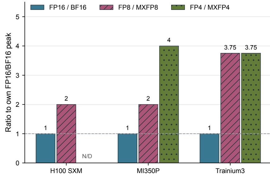
(a) Precision-dependent theoretical throughput
