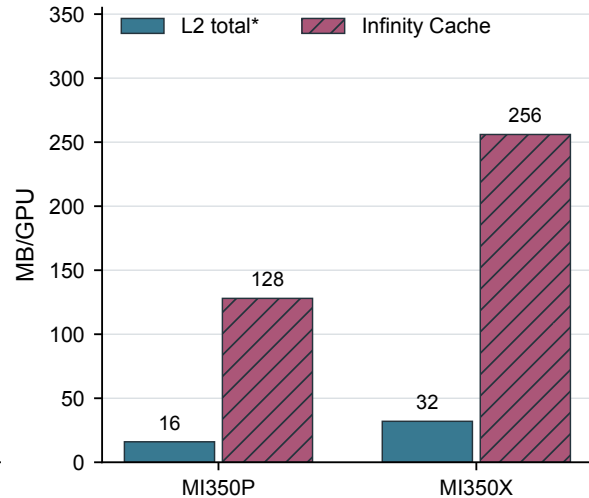
(c) Separate AMD cache levels
