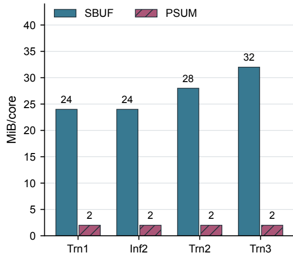
(a) AWS local work memories
