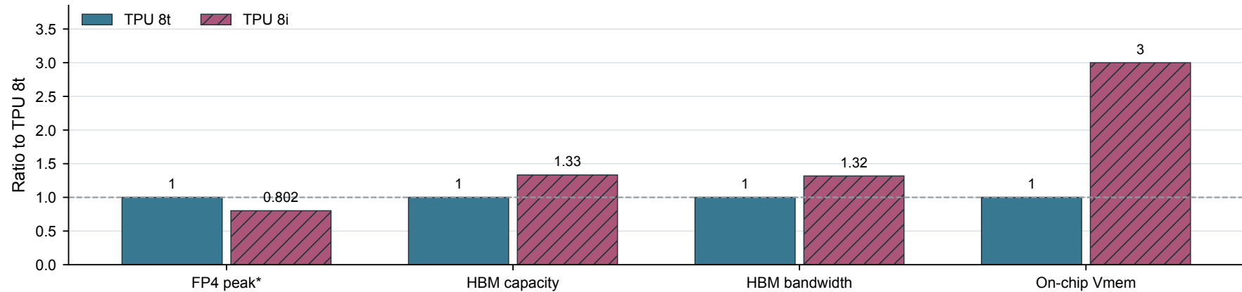
TPU 8i resource allocation relative to TPU 8t
