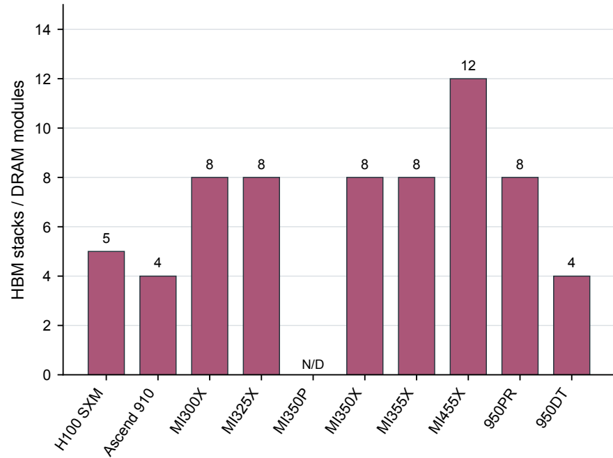
(b) Co-packaged DRAM modules
