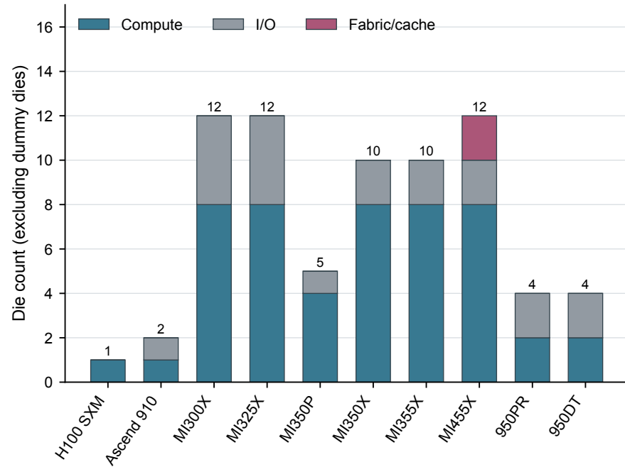
(a) Functional logic dies per package
