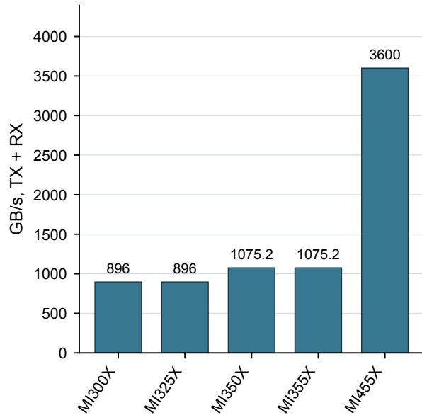
(b) AMD GPU-link endpoint
