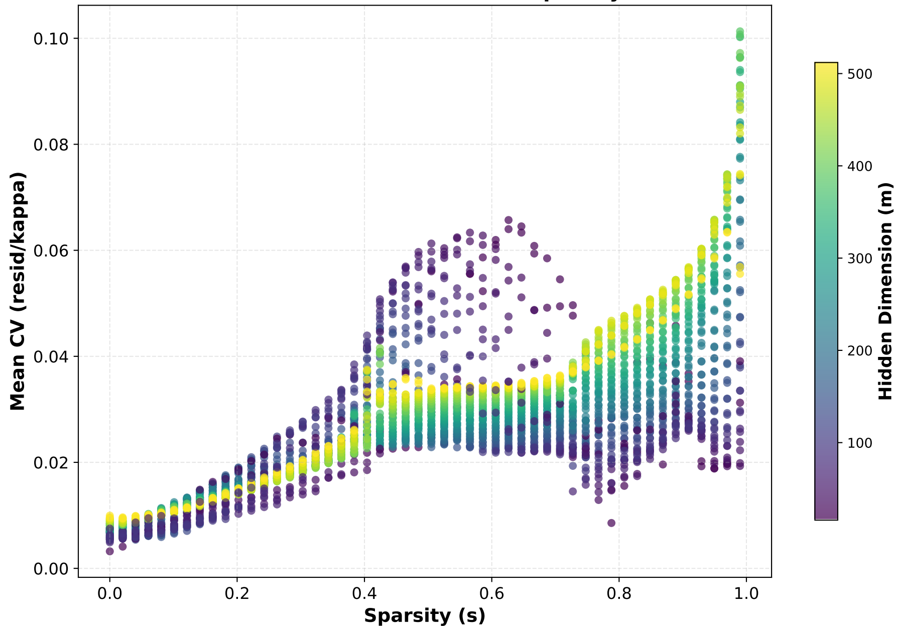
Coefficient of Variation vs Sparsity
