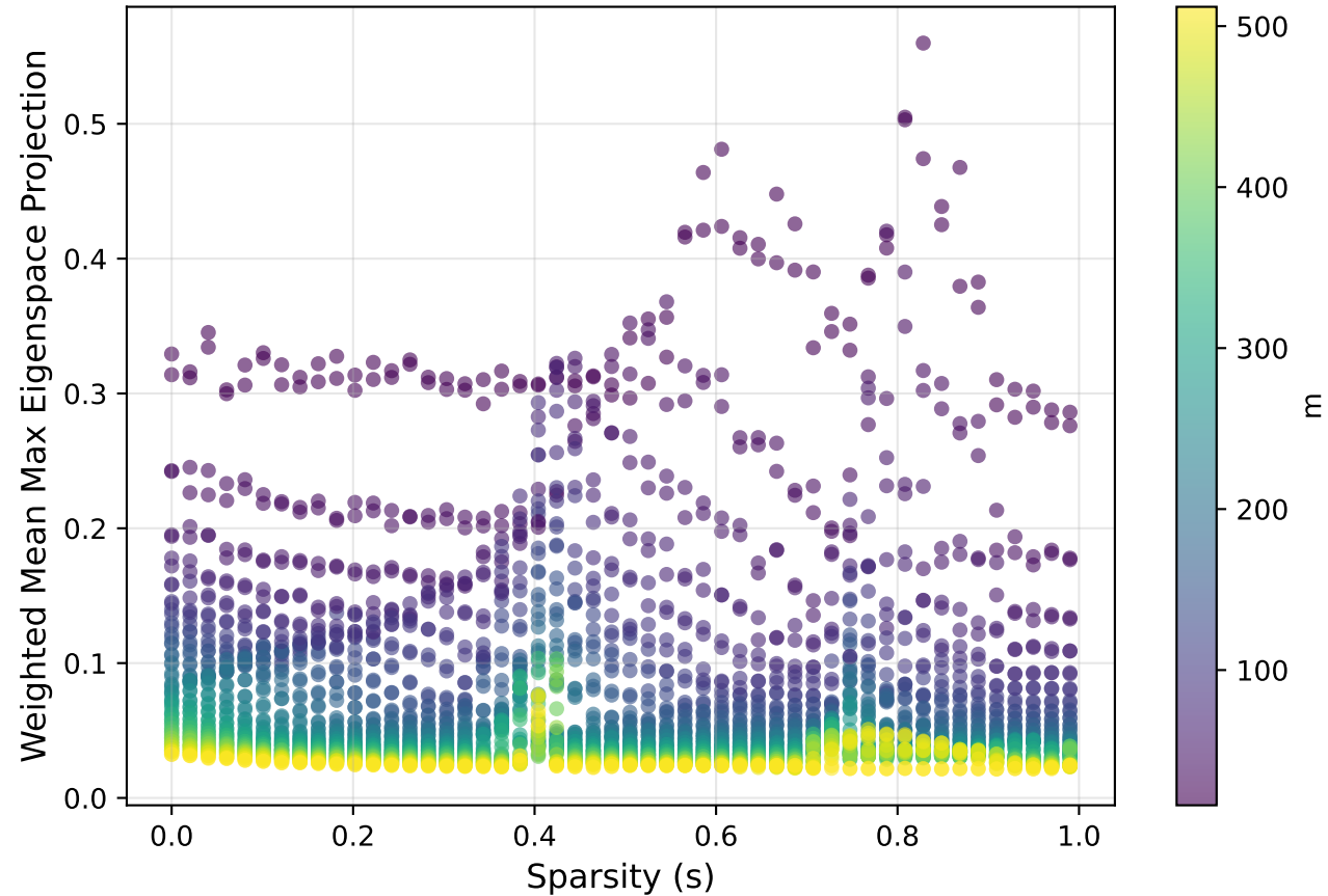
Eigenspace Localization vs Sparsity
