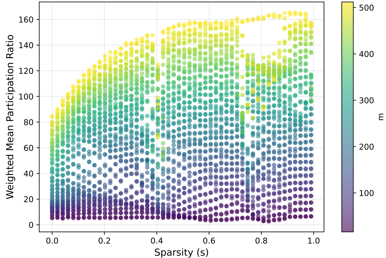
Eigenspace Delocalization vs Sparsity
