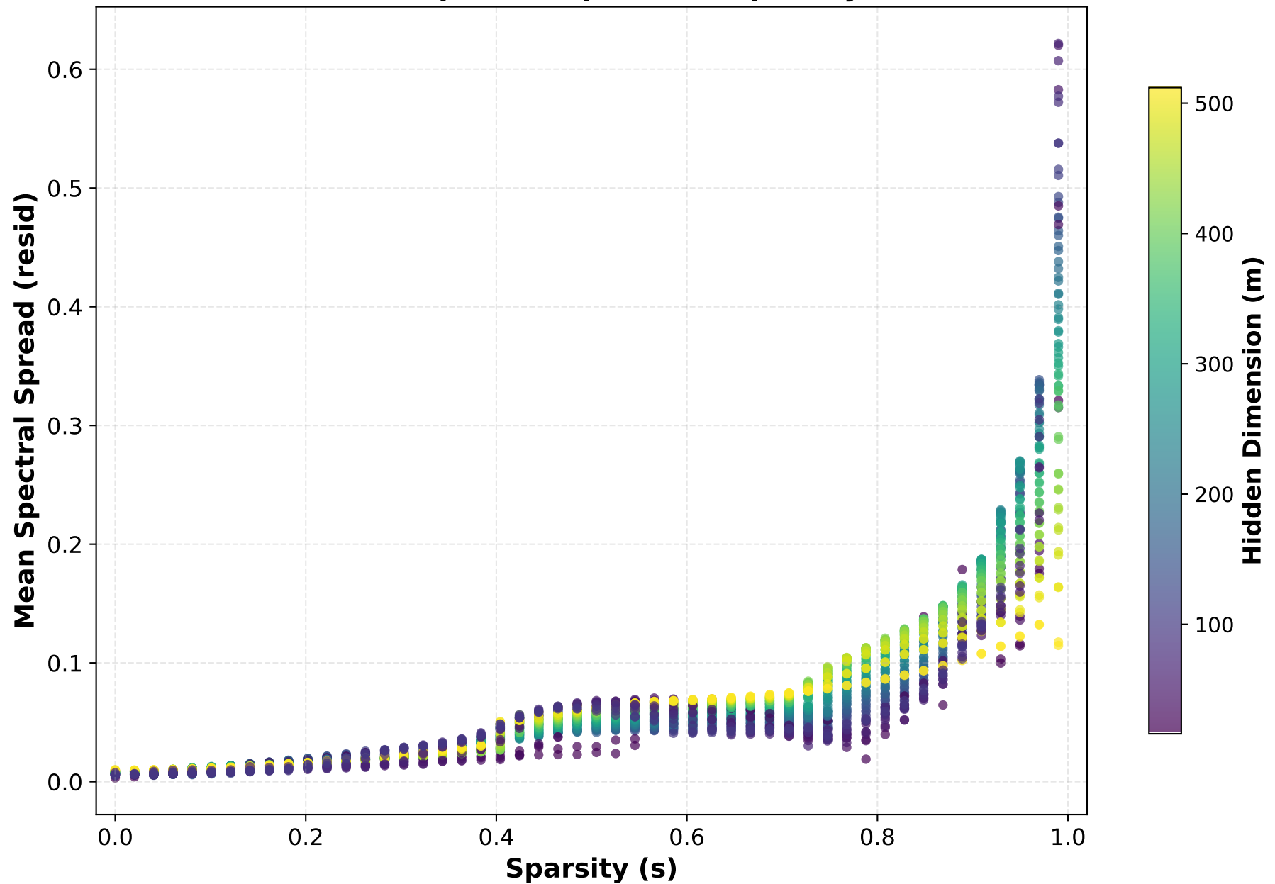
Mean Spectral Spread vs Sparsity
