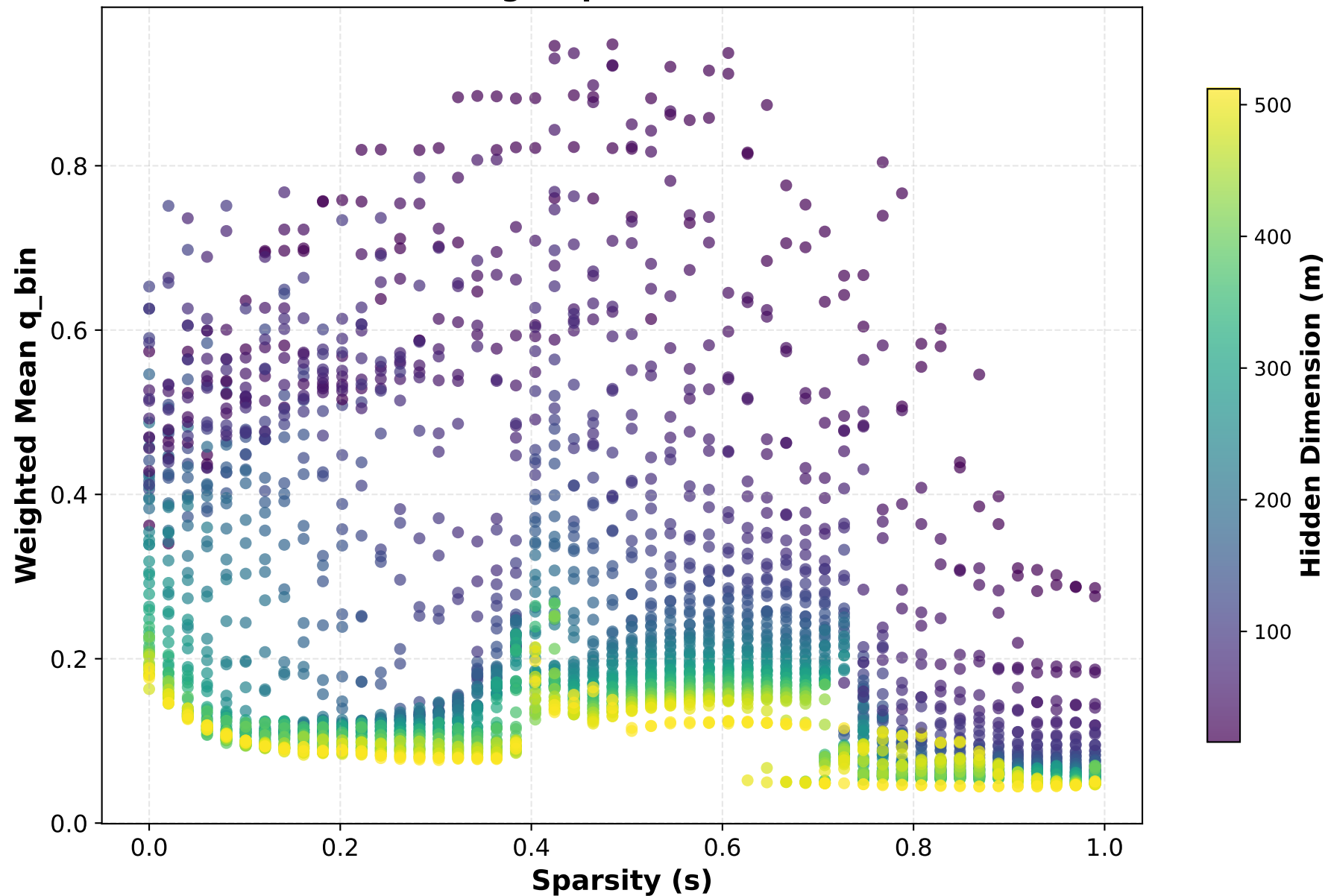
Binned Diracness Proxy vs Sparsity (Eigenspace-based)
